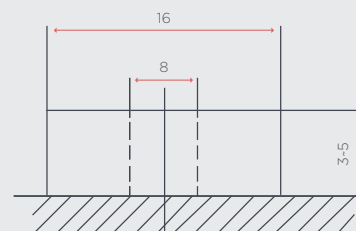
Terminal M8 Insert
